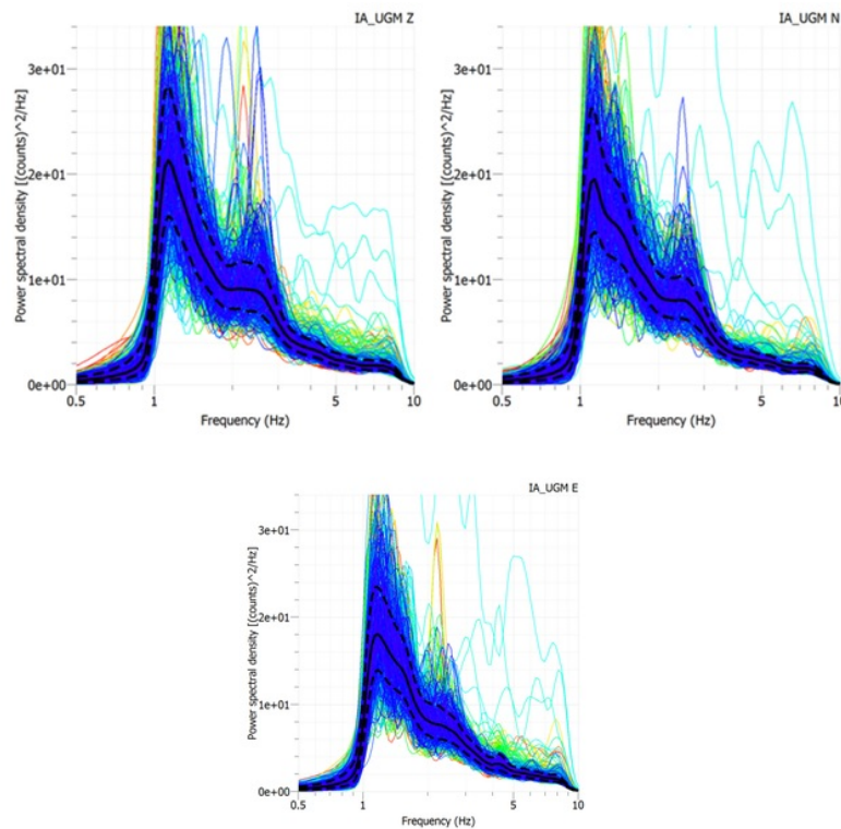
Fig. 4. Three panels of spectral amplitude analysis, showing the amplitudes of the 3 components (Z, N, E) of ambient noises with respect to the observed frequency ranges recorded by the UGM station. Many features are well understood and include microseisms in the range 0.5-10 Hz. The measured peaks of all components correspond to micro-tremor signals with frequencies of less than 2 Hz, suggesting no indication of a potential hydrocarbon reservoir above the station.
