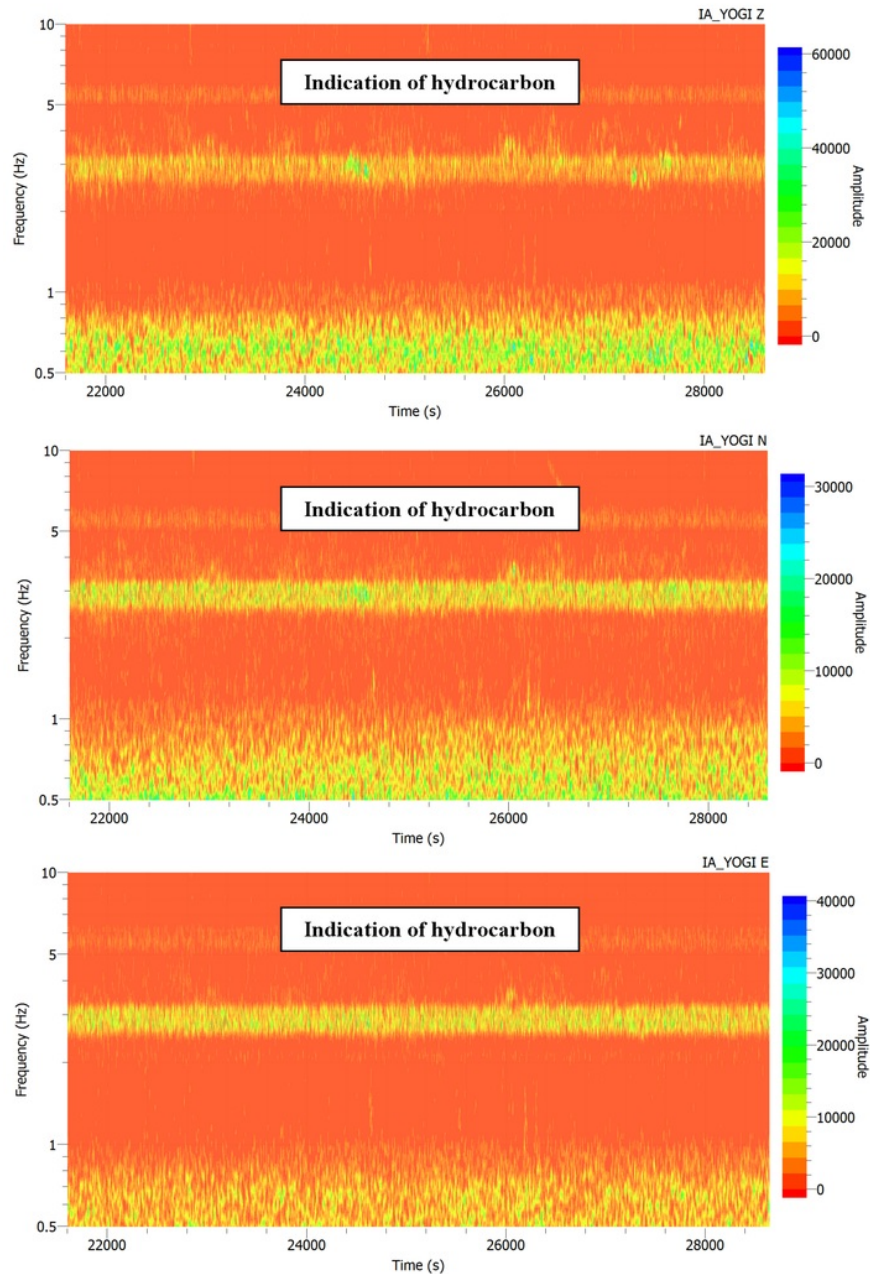
Fig. 7. Three panels of spectrogram analysis, showing spectrograms of the 3 components (Z, N, E) of ambient noises with respect to the observed frequency ranges recorded by the YOGI station. Many features are well understood as micro-tremor signals of 0.5-1 Hz and other detected signals lying between 2-4 Hz, indicating a potential hydrocarbon reservoir above the station.
