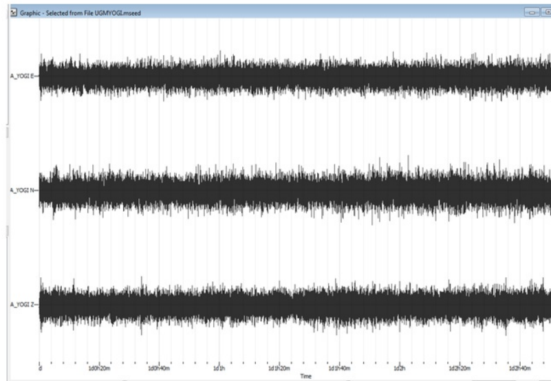
Fig. 2. Time series of 3 components (E = eastward-westward, N = northward-southward, Z = upward-downward) of broadband-noise signals recorded by YOGI station on February 19, 2017 at night from 10 pm to 5 am.
