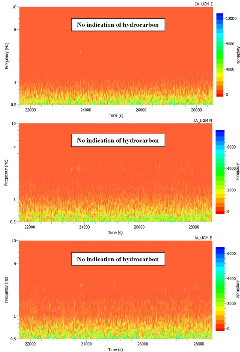
Fig. 5. Three panels of spectrogram analysis, showing spectrograms of the 3 components (Z, N, E) of ambient noises with respect to the observed frequency ranges recorded by the UGM station. Many features are well understood as micro-tremor signals of 0.5-1 Hz and possibly extended to less than 2 Hz. No signals with frequencies between 2-4 Hz indicate no potential hydrocarbon reservoir above the station.
