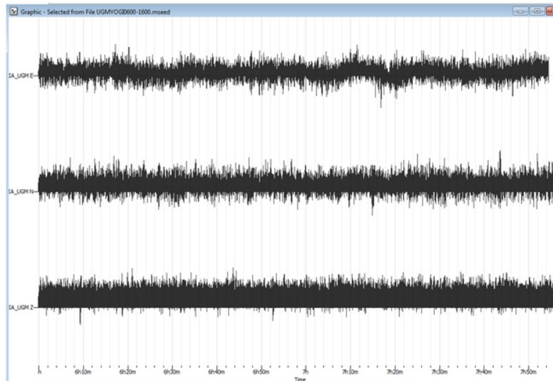
Fig. 3. Time series of 3 components (E = eastward-westward, N = northward-southward, Z = upward-downward) of broadband-noise signals recorded by UGM station on February 19, 2017 during daytime from 6 am to 4 pm.
