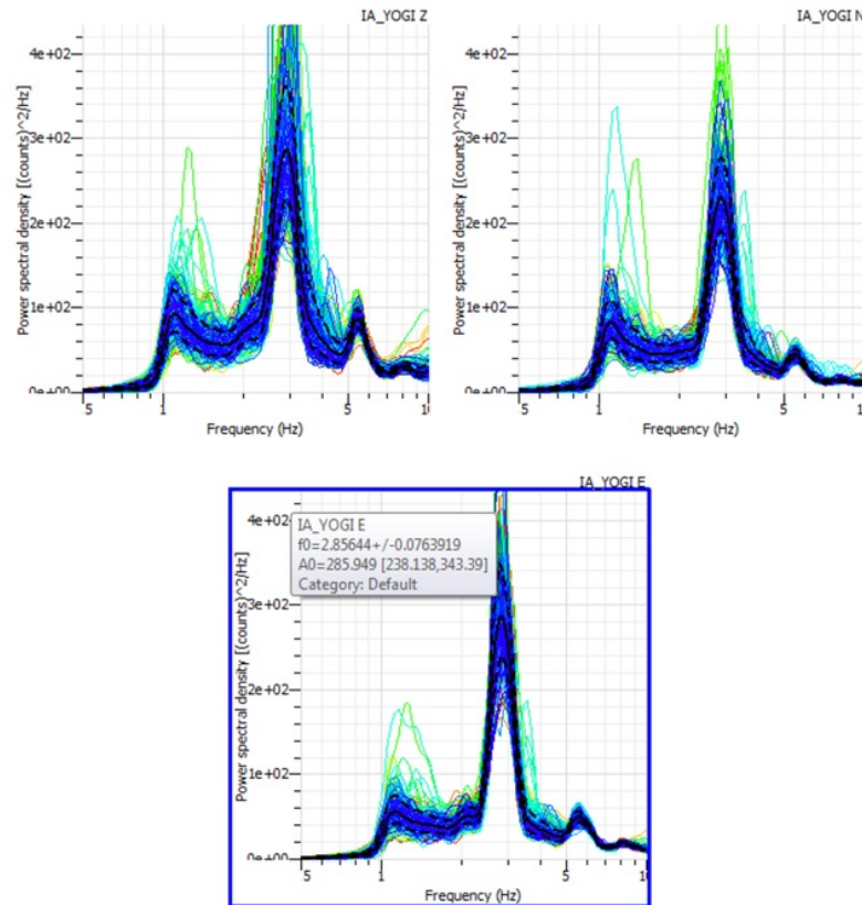
Fig. 6. Three panels of spectral amplitude analysis, showing the amplitudes of the 3 components (Z, N, E) of ambient noises with respect to the observed frequency ranges recorded by the YOGI station. Many features are well understood and include microseisms in the range 0.5-10 Hz, within which micro-tremor seismic signals of 1-6 Hz are apparently observed. The measured peaks of all components correspond to these signals with frequencies of approximately 3 Hz (see the frequency associated with the peak of power spectral density at the bottom panel), indicating a potential hydrocarbon reservoir above the station.
